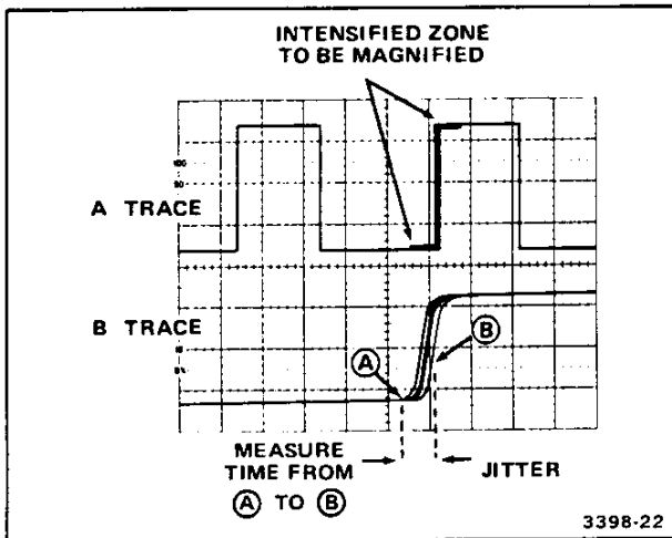
Figure 21. Pulse jitter.
