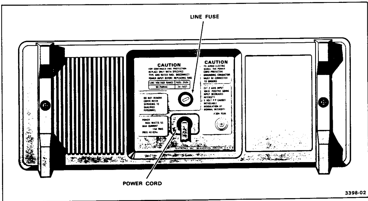
Figure 2. Line fuse and power cord.
