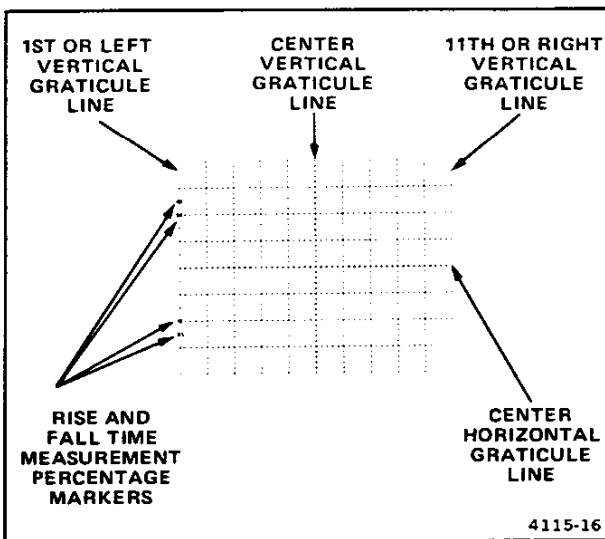
Figure 8. Graticule measurement markings.
