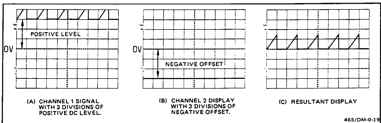
Figure 13. Algebraic addition.
