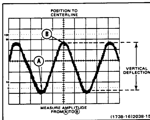
Figure 11. Peak-to-peak waveform voltage.
