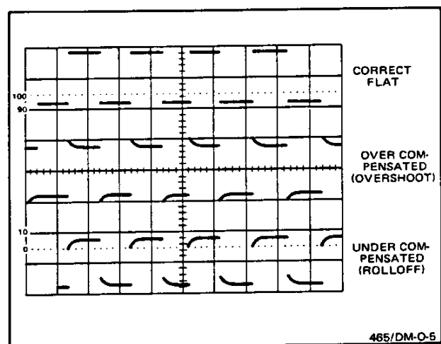
Figure 10. Probe compensation.
