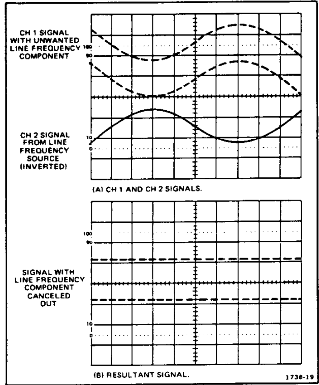
Figure 14. Common-mode rejection.
