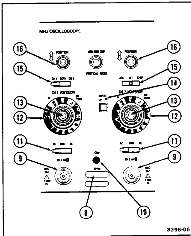
Figure 4. Vertical controls and connectors.
